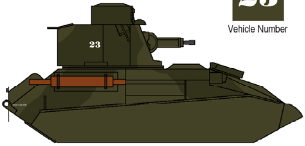
Light Tank Mk.VIb 'T1223' - The Canadian Armoured Vehicle Training Centre, Camp Borden, Ontario, 1940
