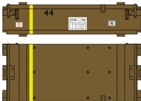
17 Pounder Ammunition Case C274 Mk.I (wood) containing 2 rounds of A.P., A.P.C., H.E. or Practice (yellow band denotes)
